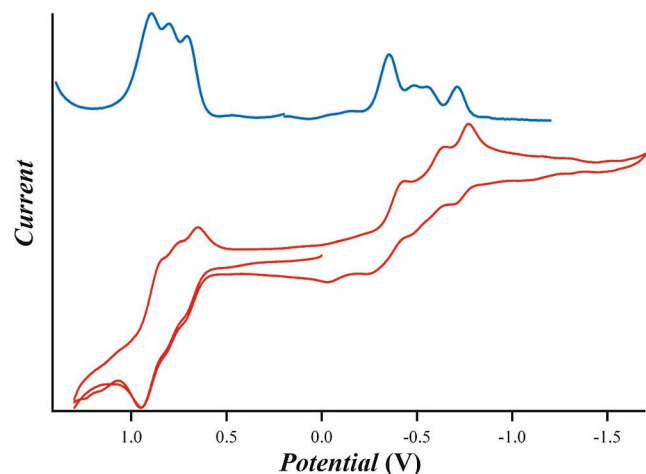
Figure 5. Electrochemical response (top: DPV, bottom: CV) of [\{\text{CoCl}\}_4\{\text{Re}(\text{triphos})(\text{CN})_3\}] ( 6 ) recorded in 0.1 M [\text{tBu}_4\text{N}][\text{PF}_6]/\text{CH}_3\text{CN} . Potentials reported vs Ag/AgCl reference electrode.
