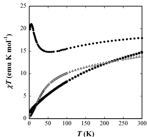
Figure 8. Temperature-dependent magnetic susceptibility data for [\{\text{MnCl}\}_4\text{-}\{\text{Re}(\text{triphos})(\text{CN})_3\}_4] ( 2 ), [\{\text{FeCl}\}_4\text{-}\{\text{Re}(\text{triphos})(\text{CN})_3\}_4] ( 4 ), and [\{\text{CoCl}\}_4\text{-}\{\text{Re}(\text{triphos})(\text{CN})_3\}_4] ( 6 ) recorded in the range of 1.8–300 K.
